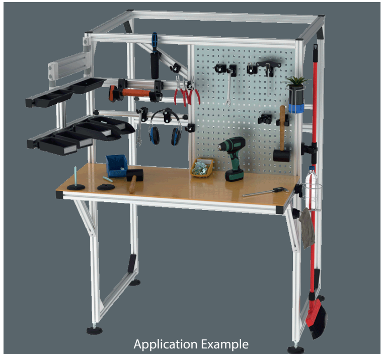
Tool Hook 7/38 - 24 Item No.: 07.01816.00
